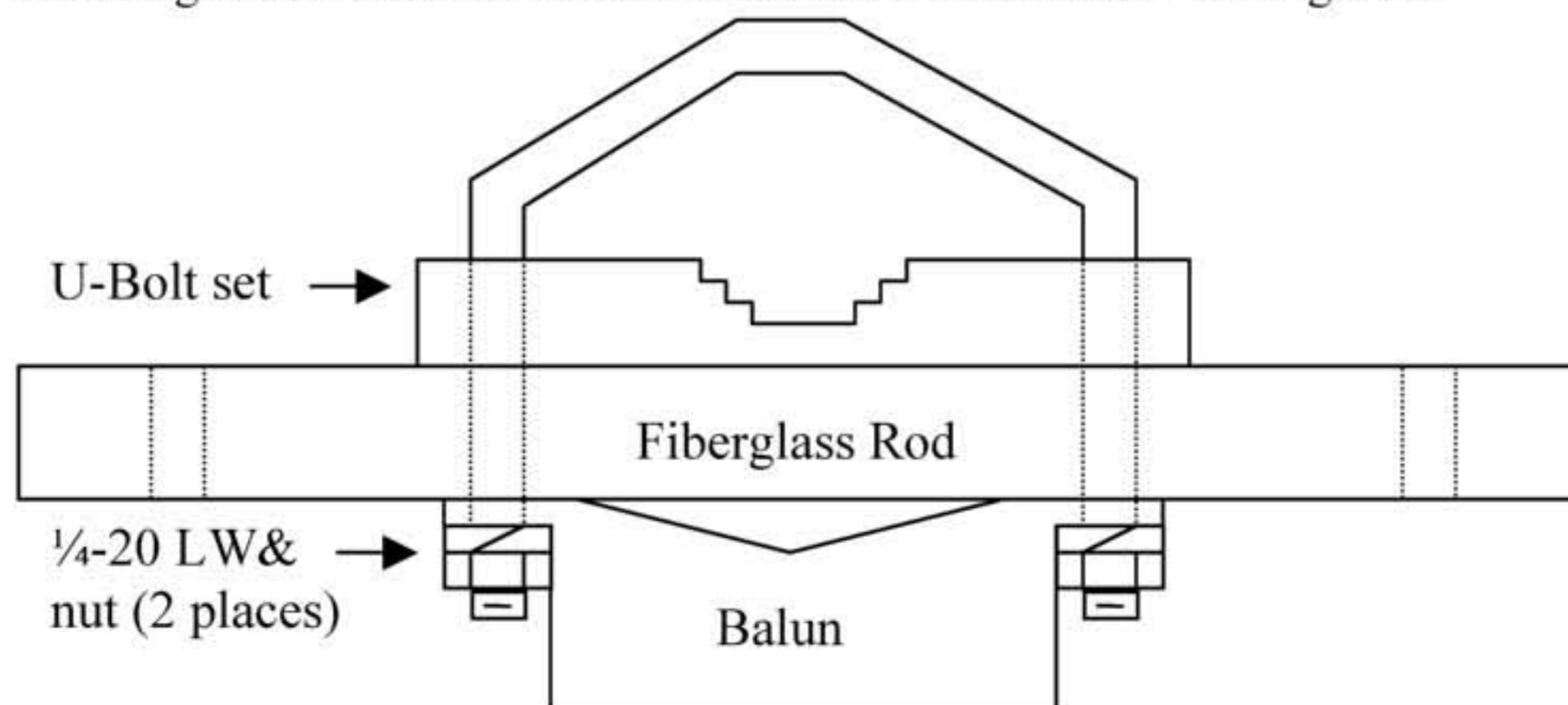
Figure 2: Balun/Center Insulator Assembly – Top View
