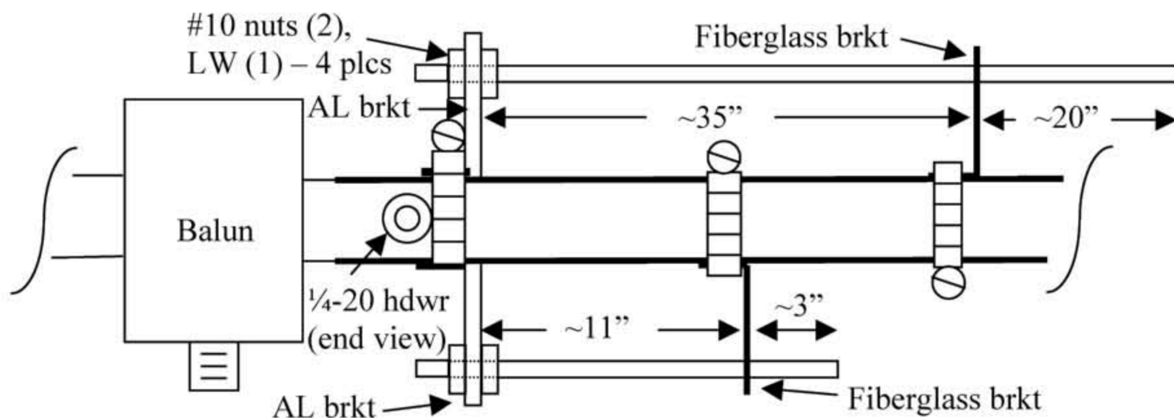
Figure 4: 6 and 2-meter stub assembly and mounting
