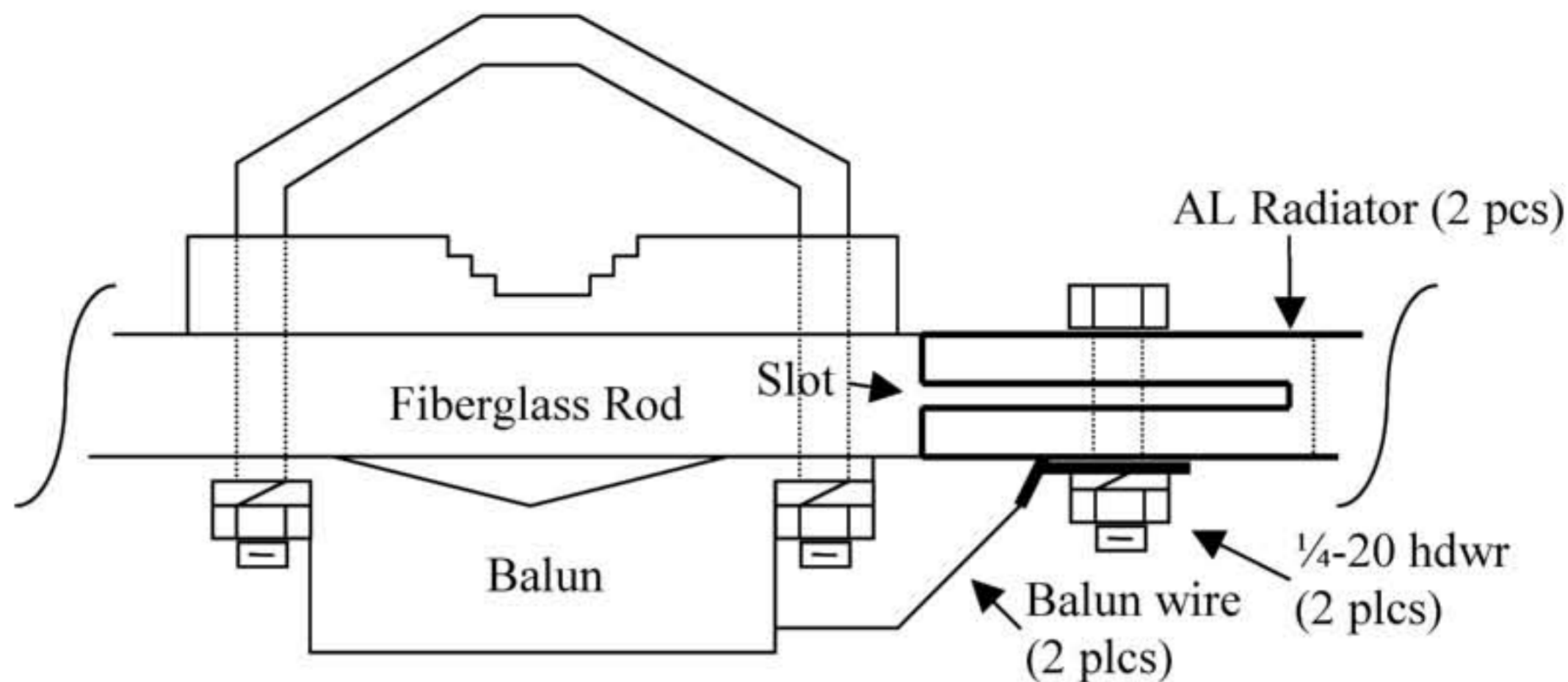
Figure 3: Radiator Tube Assembly – Top View
